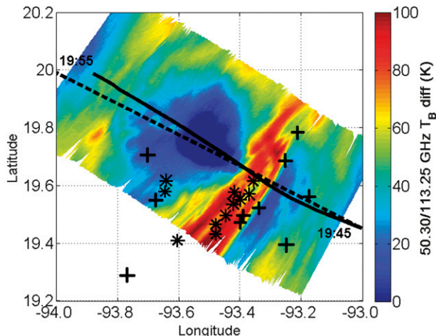
FIG. 10. The T_B differences between the 50.30- and 113.25-GHz channels of HAMSAR from 1945 to 1955 UTC. Large T_B differences (red) in the southeast eyewall indicate regions where greater ice scattering, and thus deep convection, are occurring. WLLN [asterisk (*)] and GLD360 [plus (+)] flashes from 1945 to 1955 UTC, as well as GH (solid) and DC-8 (dashed) flight tracks, are overlaid for reference.
